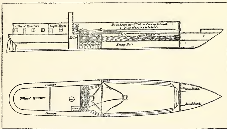
DIAGRAM OF THE POWDER-BOAT LOUISIANA.
